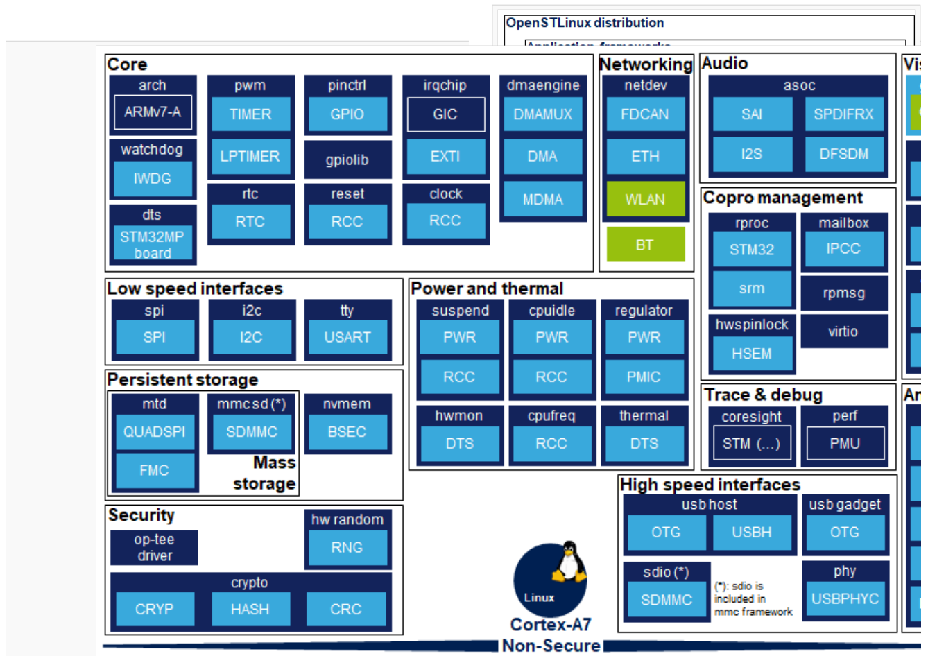
STM32MP15 Linux kernel overview
