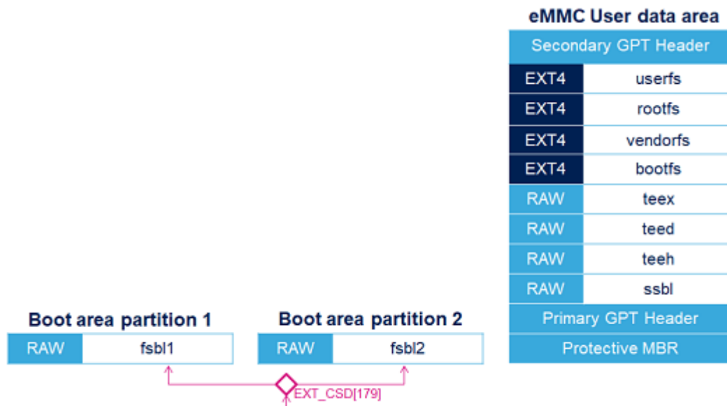
The ROM code gets the FSBL copy from the boot partition selected by the eMMC EXT_CSD[179] register.
