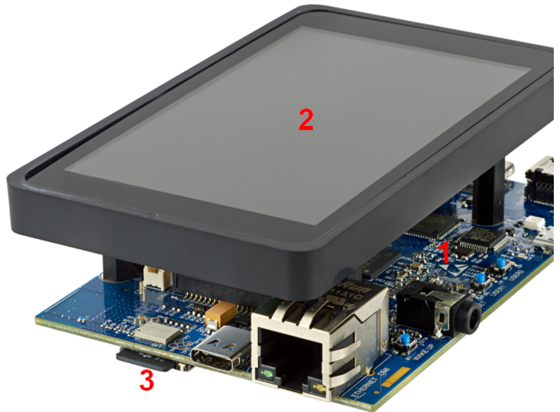
STM32MP157x-DKx Discovery kit assembled STM32MP157C-DK2 shown here (picture not contractual) (for the STM32MP157A-DK1, the element 2 is not present)
