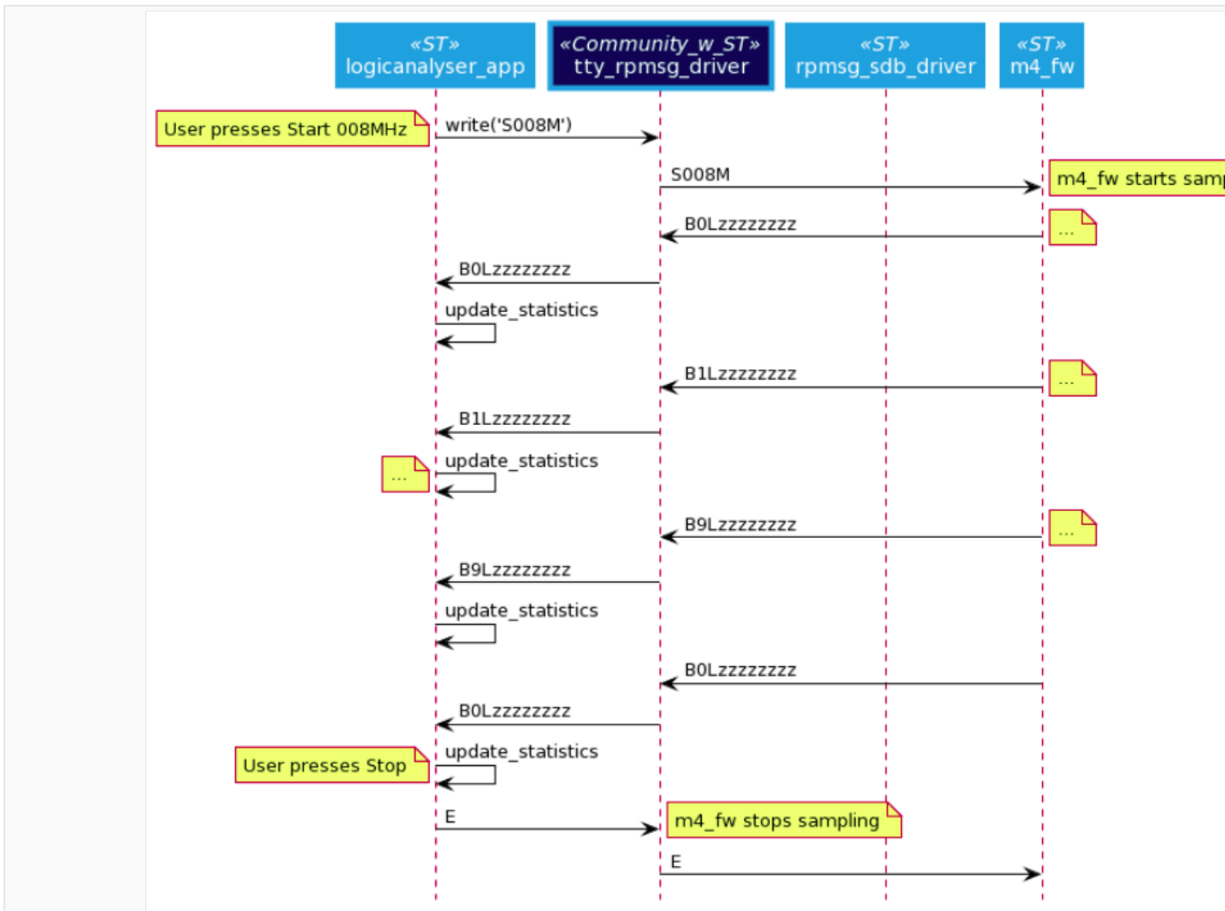
Sampling frequency more than 5 MHz
