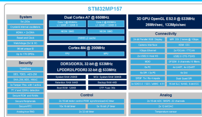
[[STM32MP15 microprocessor|Template:Blue]]
