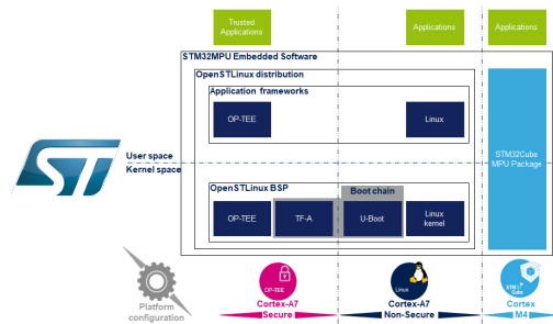
STM32MPU Embedded Software architecture overview
