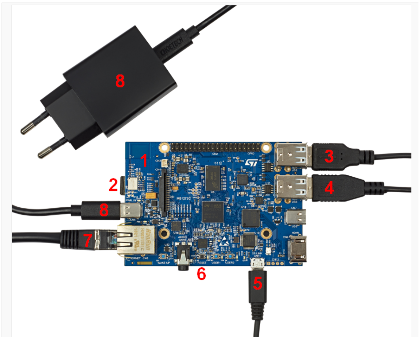
STM32MP157x-DKx Discovery kit connections
